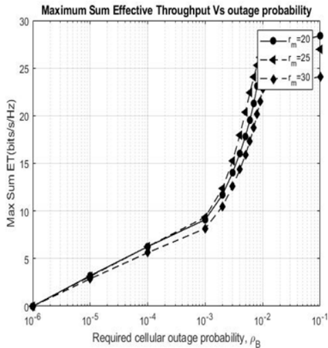
Fig. 5: Maximum Sum effective throughput Vs Outage probability
